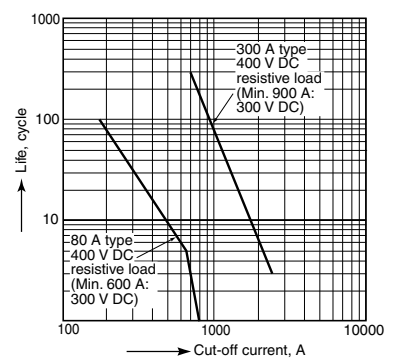
4. Cut-off life curve
