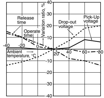
1-(3) Ambient temperature characteristics (300 A)
