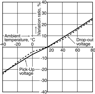
1-(1) Ambient temperature characteristics (10 A)
