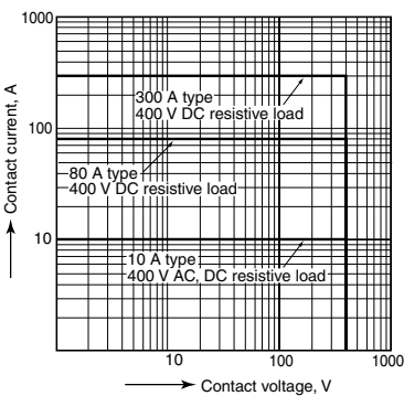
2. Max. value for switching capacity
