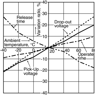
1-(2) Ambient temperature characteristics (80 A)
