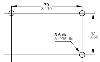
Mounting dimensions
