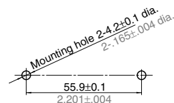
Mounting dimensions
